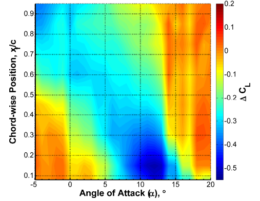
Figure 5: Contour of change in lift coefficient for h/c = 0.02 . stall angles, a leading-edge location is preferable.
